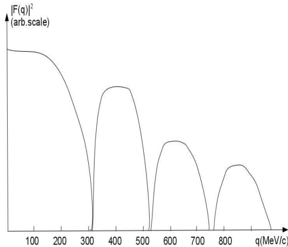
FIGURE 1 – Form factor of ^{14}\text{N} as a function of the transferred momentum during the scattering.
