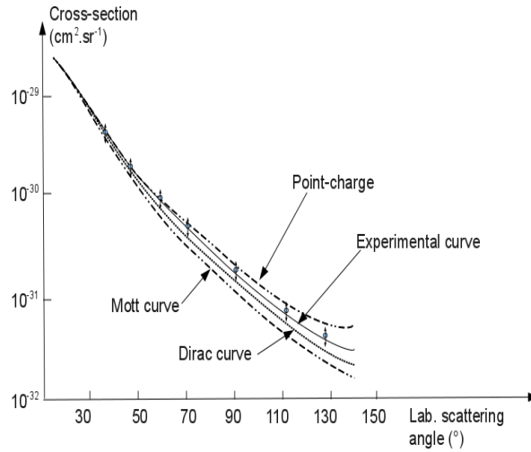
FIGURE 2 – Differential cross section of electrons on H_2 versus the scattering angle \theta .
